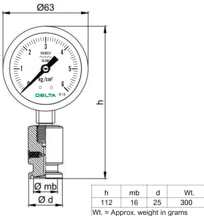
Dimensional Drawing
